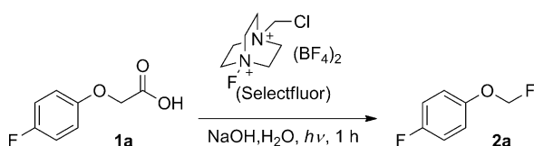
Scheme 1. Photo-fluorodecarboxylation of the \alpha -aryloxy derivative 1a .
