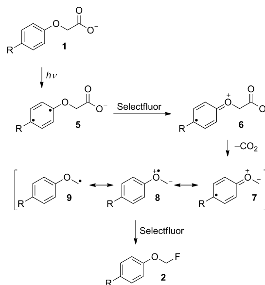
Scheme 3. Current working mechanistic model. [14]
