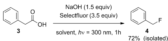
Scheme 2. Photo-fluorodecarboxylation of phenylacetic acid ( 3 ).
